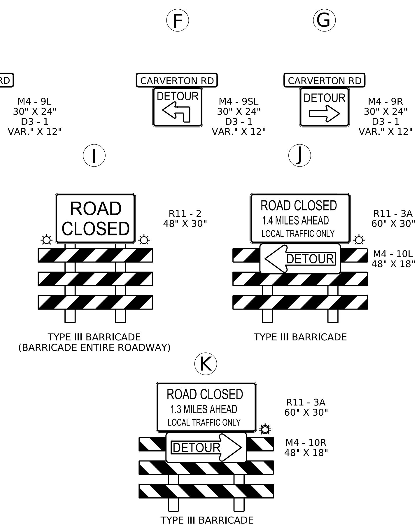
TABULATION OF TRAFFIC CONTROL DEVICES (FOR INFORMATION ONLY)
