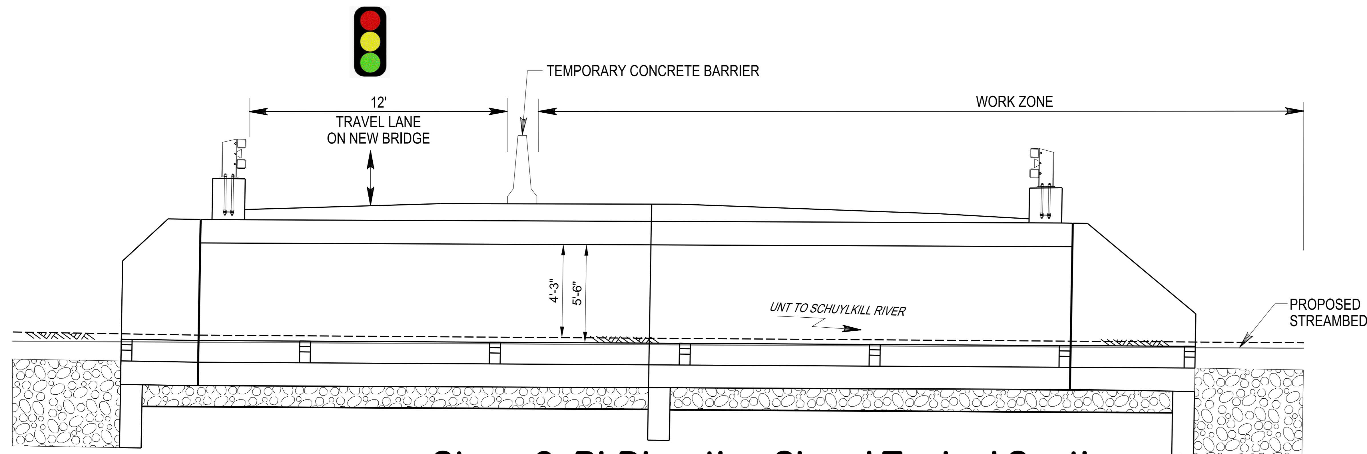
Stage 2- Bi-Direction Signal Typical Section
