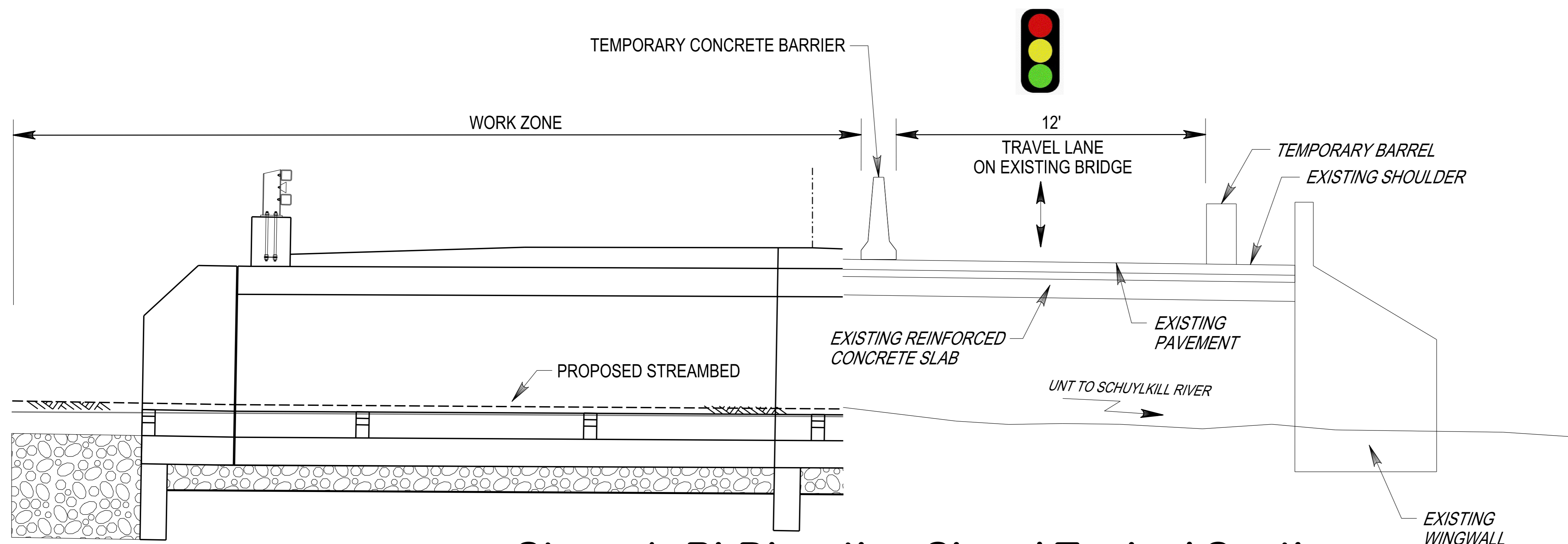
Stage 1- Bi-Direction Signal Typical Section
