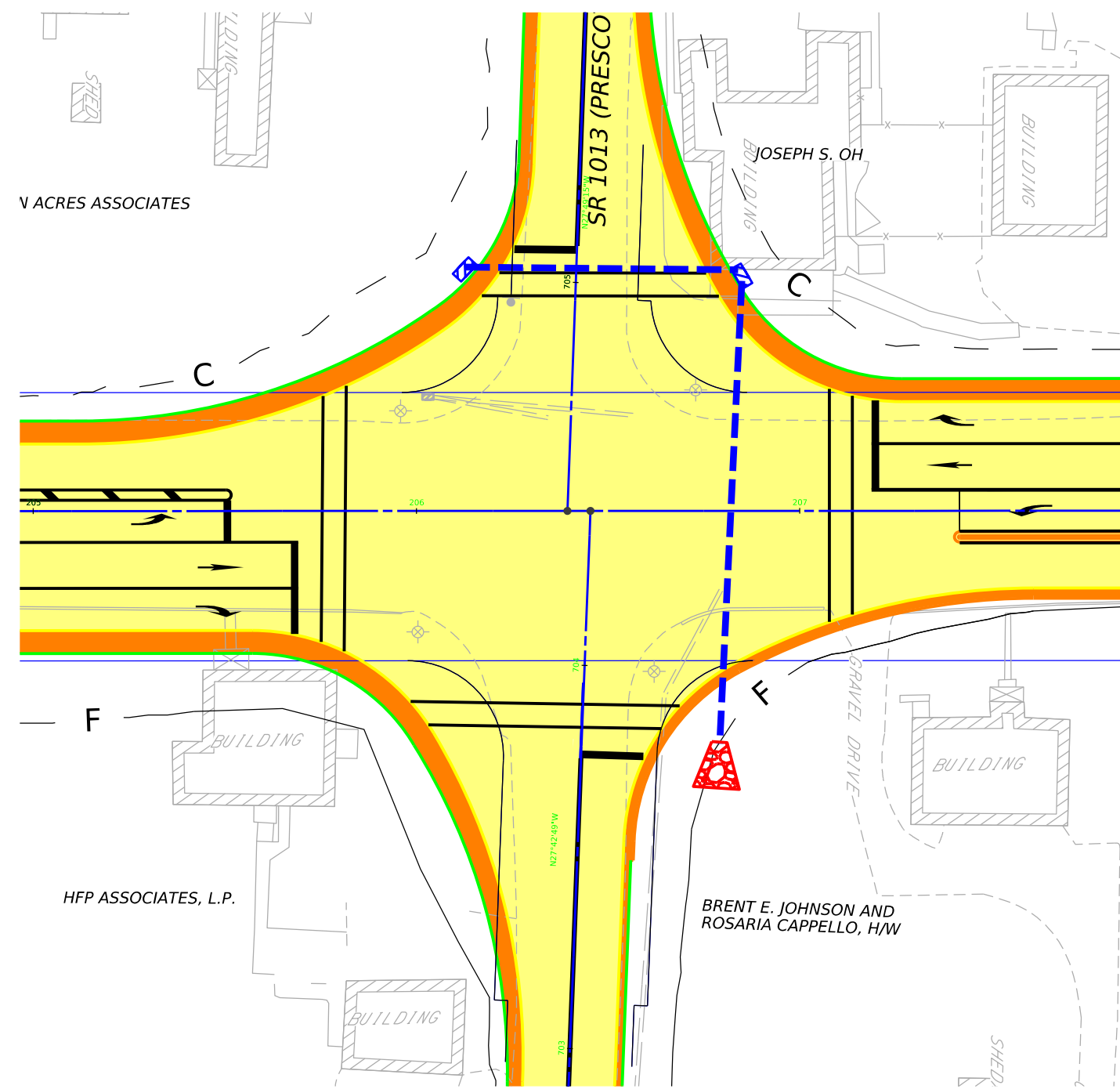
INTERSECTION DETAIL (NOT TO SCALE)
