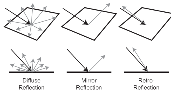
Exhibit 2-1 Types of Retroreflection
