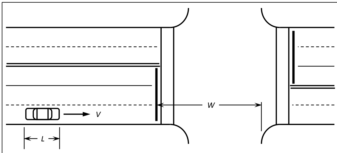
Exhibit 4-20 Definition of Terms for All-Red Clearance Intervals
