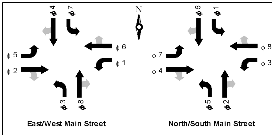
Exhibit 4-26 Traffic Signal Phase Numbers
