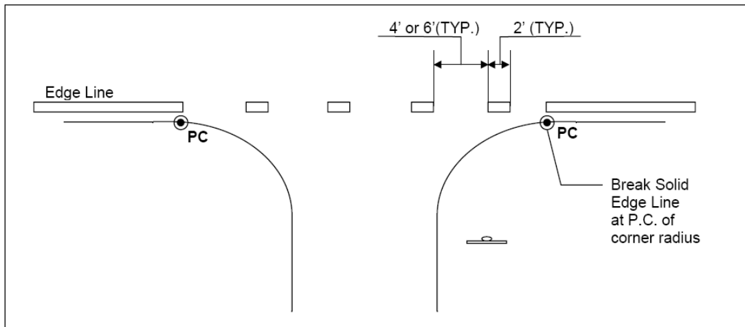
Exhibit 3-3 Dotted White Edge Lines
